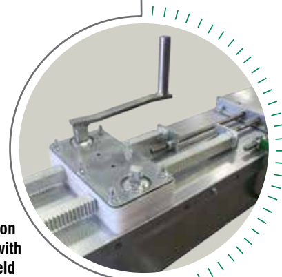
Rack and Pinion Opener
